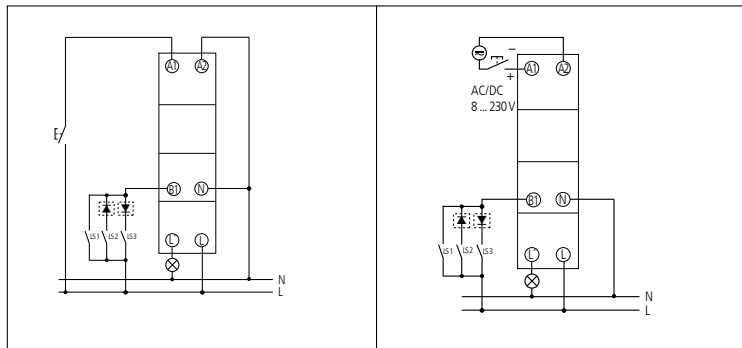
Raccordement 230 V
