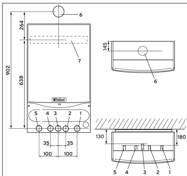
Fig. 3.5 Dimensions de raccordement
