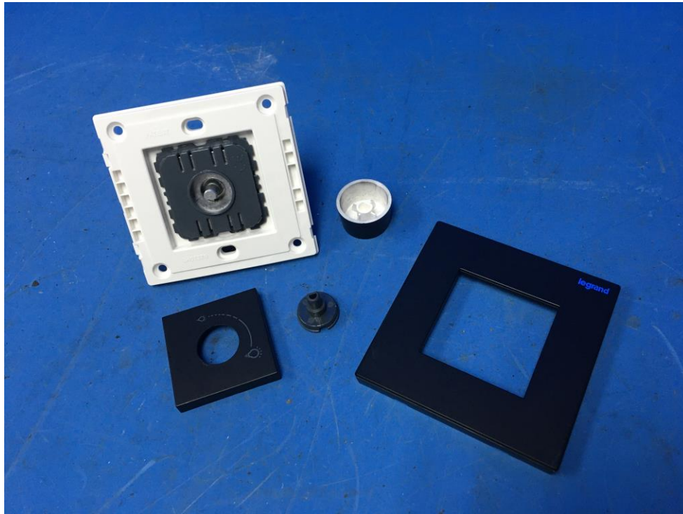
Exploded view I of 282419 series
