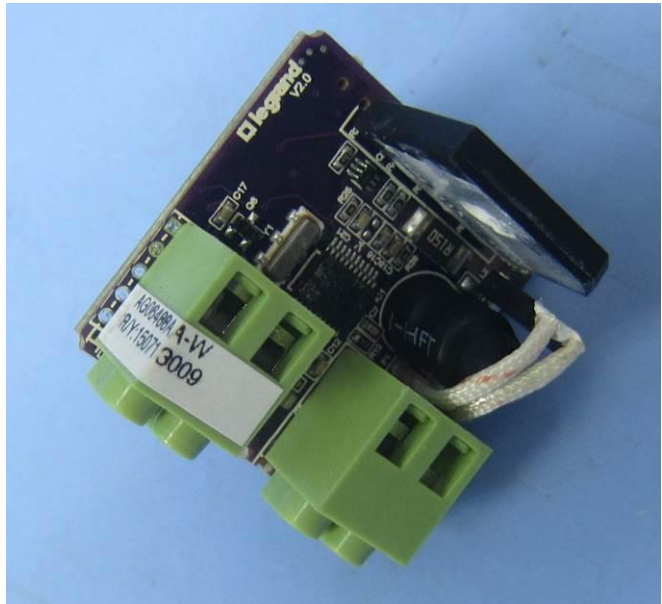
PCB view detail of model CXM17
