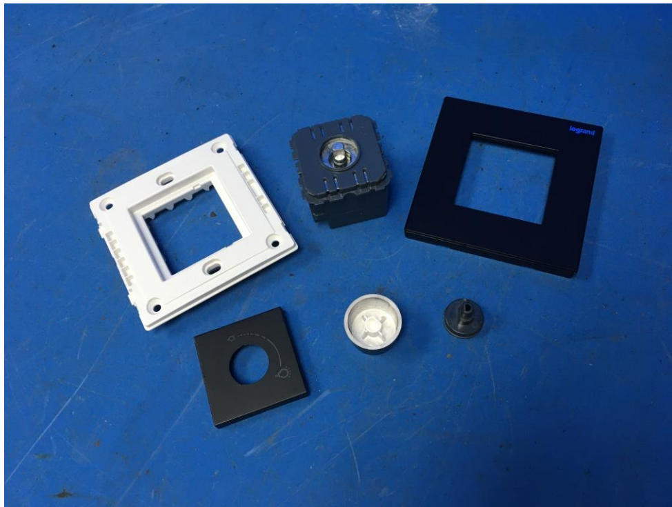
Exploded view II of 282419 series
