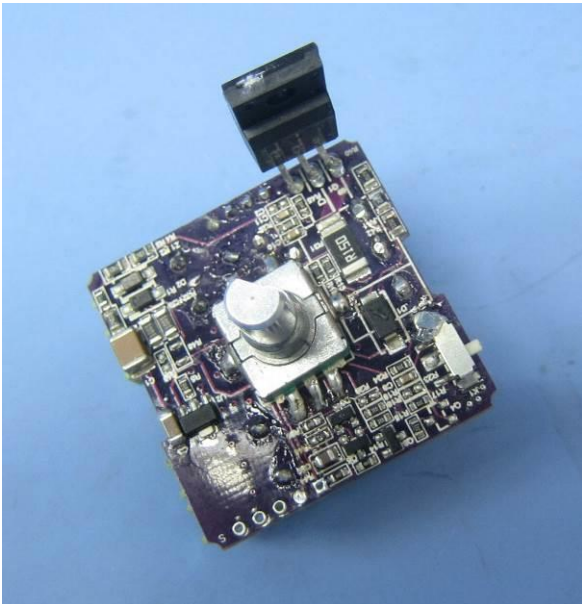
PCB view detail of model CXM17
