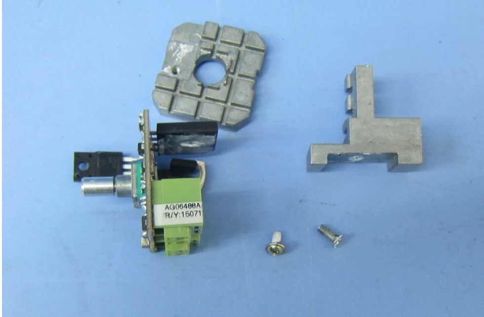
Electrical parts view of model CXM17 after heat sink removed
