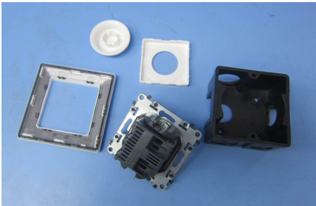
Exploded view III of mounting box (for example) for AG05476AA; AG06488AA
