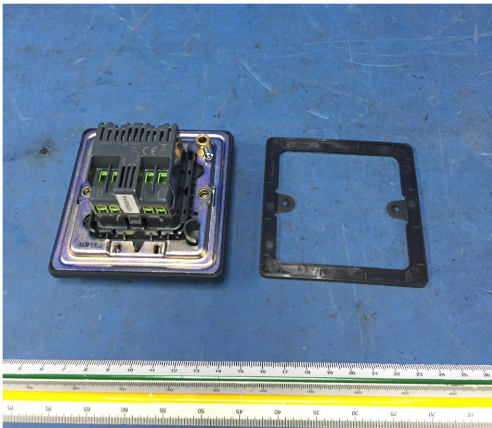
Model 833151, same as 832151
